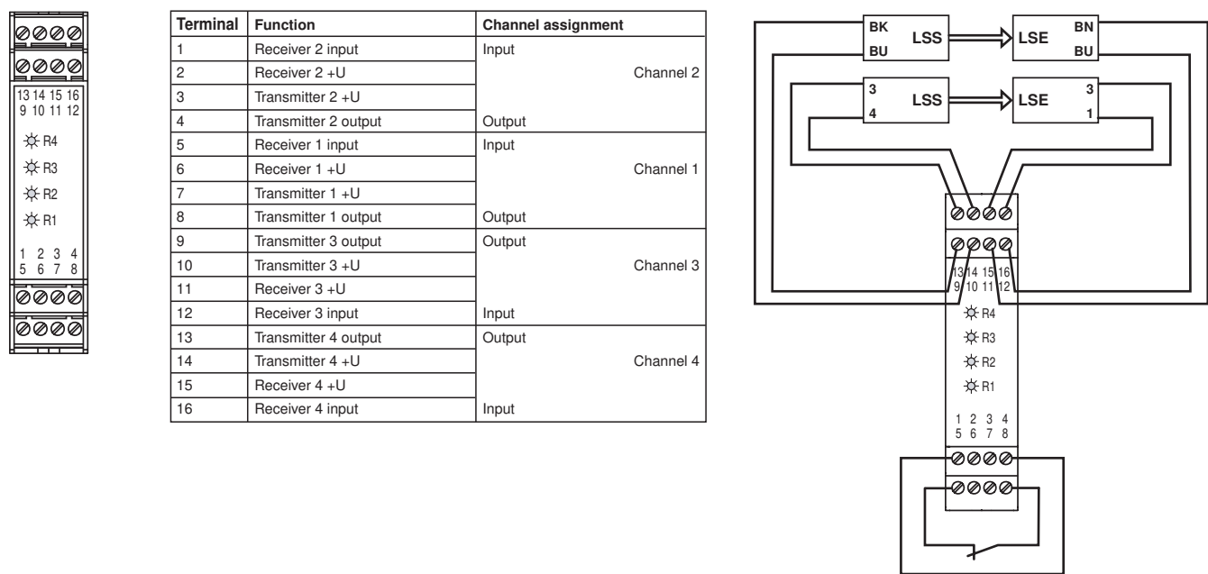
Connection example (LSS = transmitter of light barrier; LSE = receiver of light barrier)
