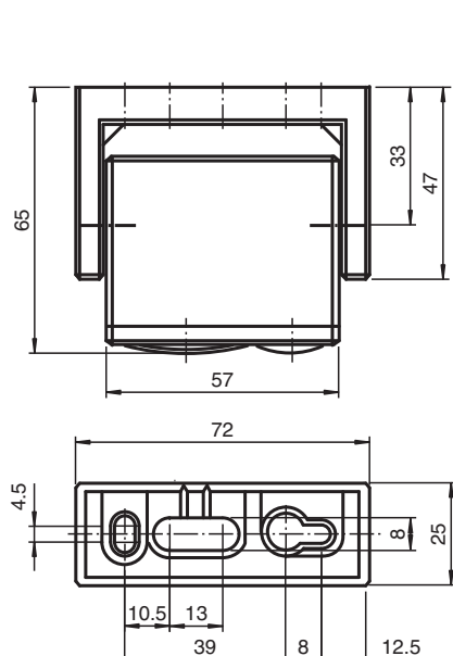
Dimension with swivel bracket
