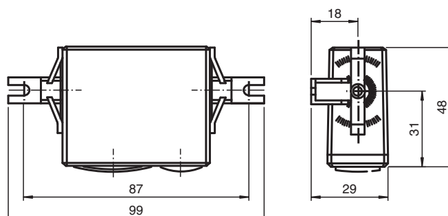
Dimensions with mounting angle
