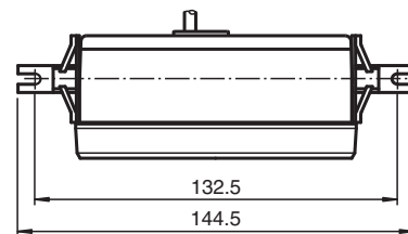
Mounting dimensions with mounting bracket set AIR30
