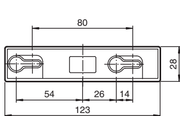
Mounting dimensions for swivel
