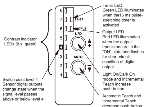
Figure 3. Push-buttons and Status Indication LEDs
