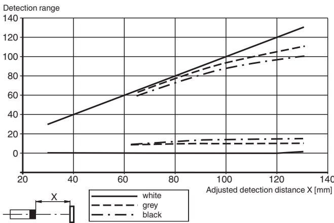
Detection range
