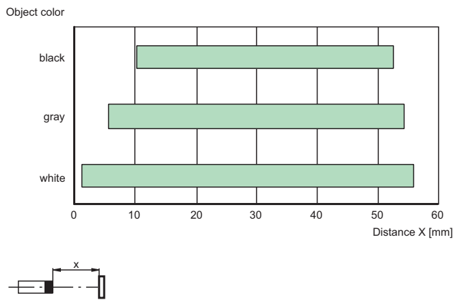
Detection ranges
