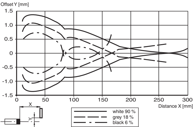
Detection ranges
