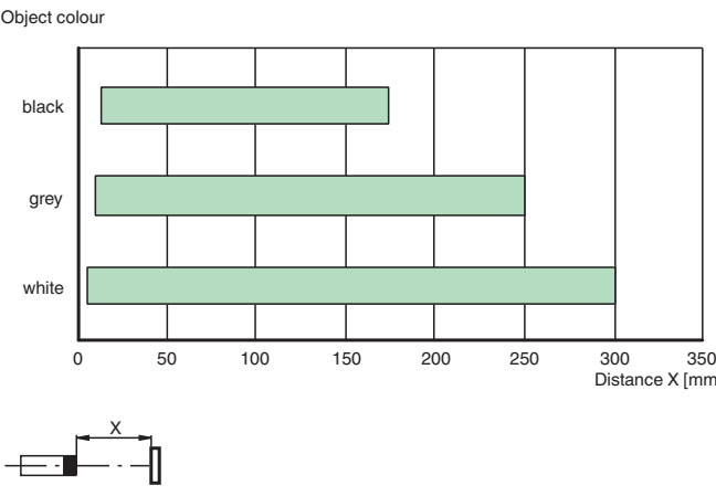
Detection ranges
