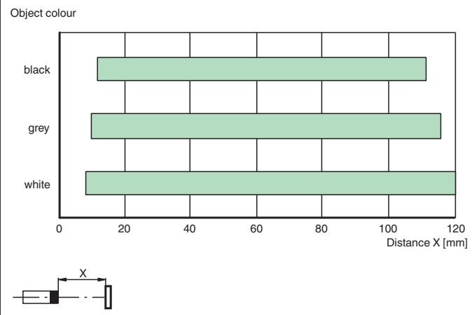
Detection ranges
