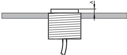
Minimum 'free zone' requirements of the WIS transmitters when installed in metal
