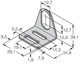
Mounting bracket for threaded barrel sensors; material: Stainless steel A2 1.4301 (AISI 304)
