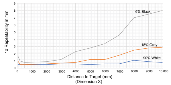
Repeatability (250 ms)
