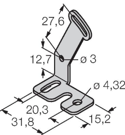
Mounting bracket, stainless steel, for 18 mm thread
