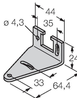
SMB30SC
